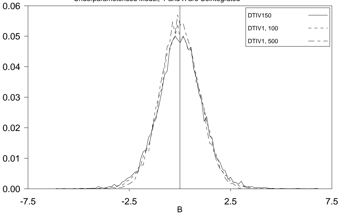
Underparameterised Model, Y and X are Cointegrated
