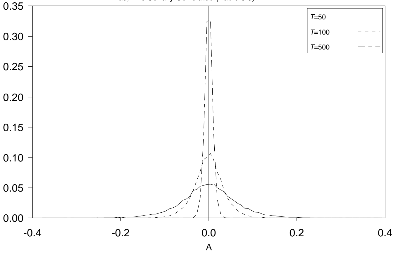
Bias, X Is Serially Correlated (Table 8.3)
