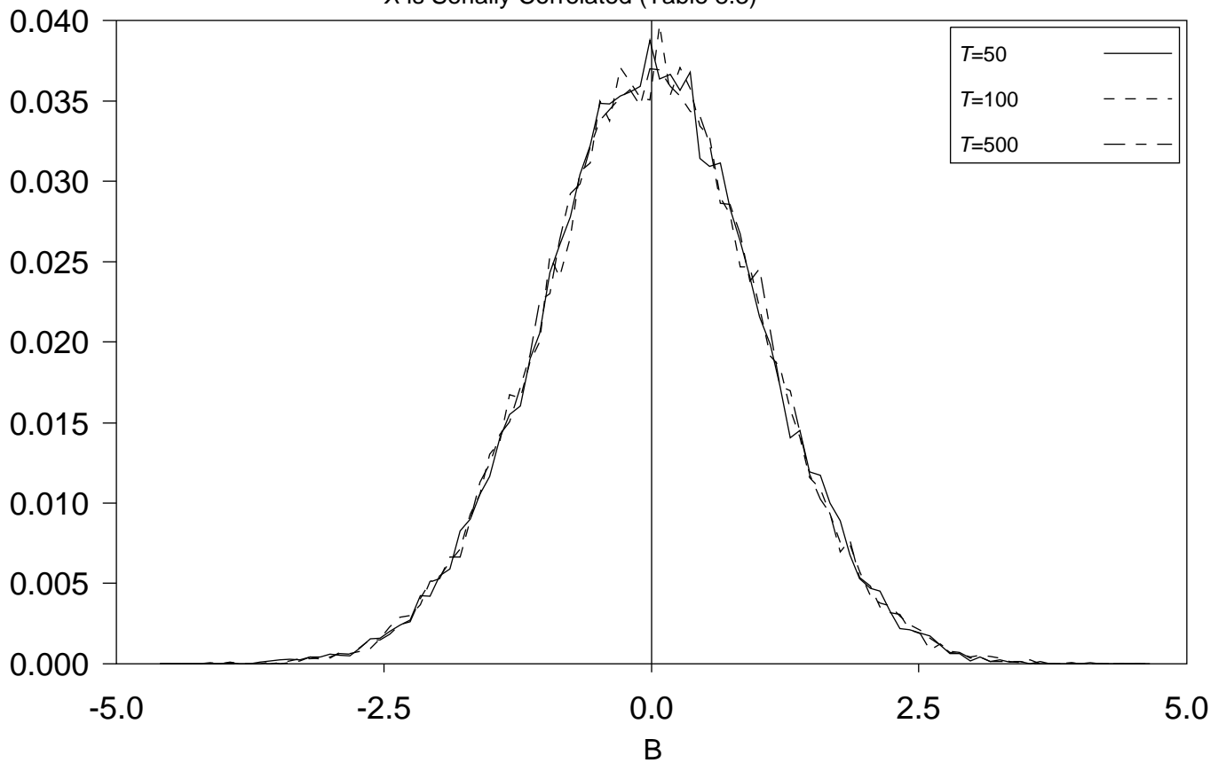
X is Serially Correlated (Table 8.3)
